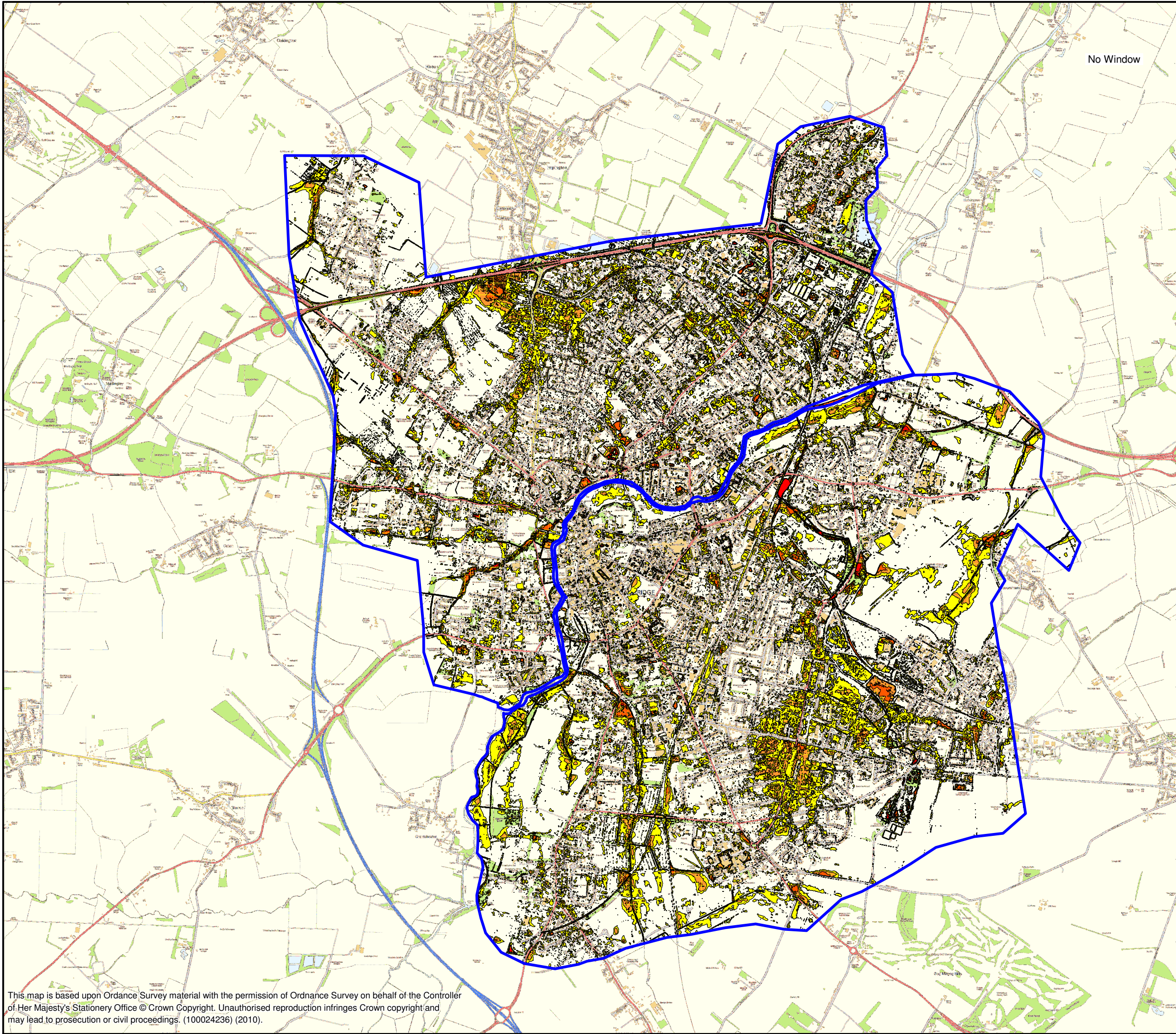
FIGURE E1 0.5% AEP "DO NOTHING" PLUVIAL MODELLING MAXIMUM DEPTH CAMBRIDGE
